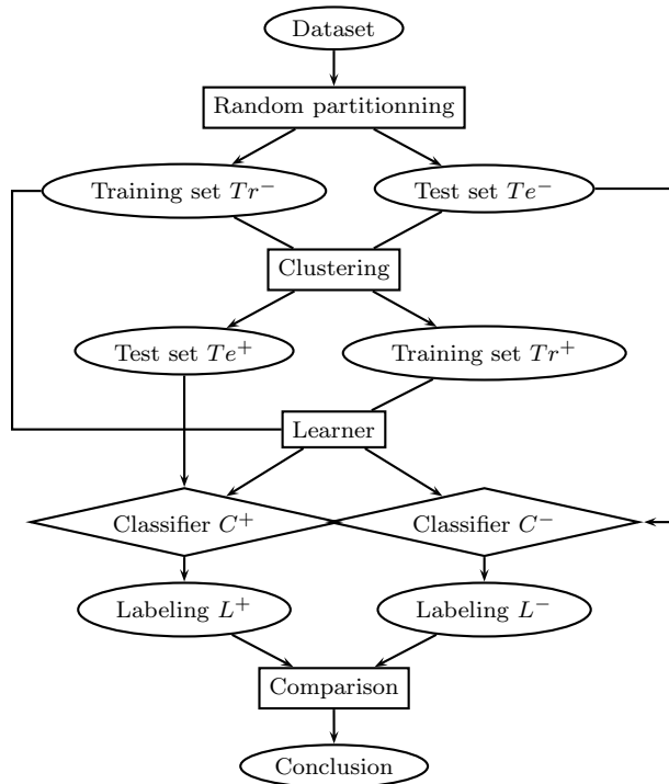
Figure 1: Methodology for evaluating the interest of adding to a dataset new information coming from a clustering algorithm.
